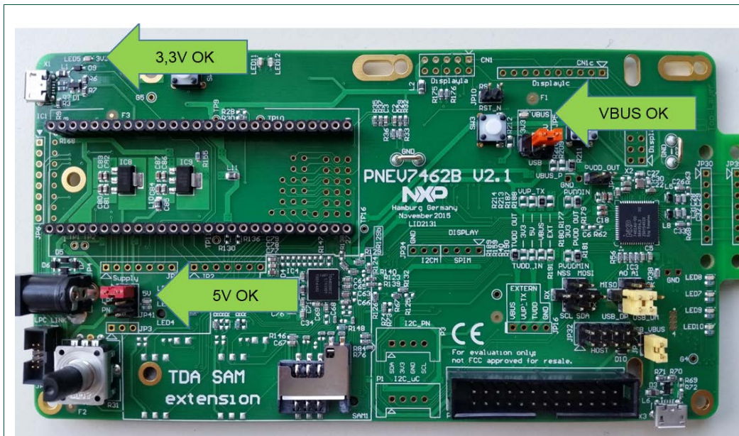
Fig 16. Supply indicator
