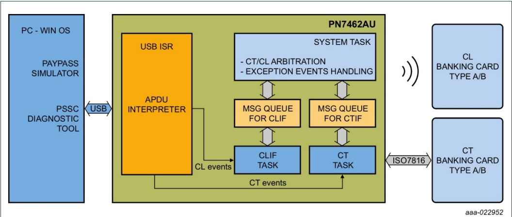
Fig 97. Example architecture
